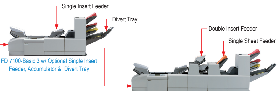
FD 7100-Basic 3 w/ Optional Single Insert Feeder, Double Insert Feeder, Single Sheet Feeder, Accumulator & Divert Tray
